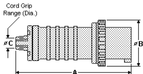
60A, 100A Plug
