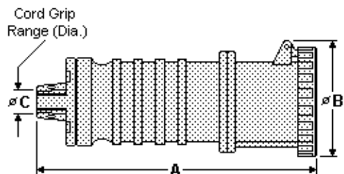
60A, 100A Connector
