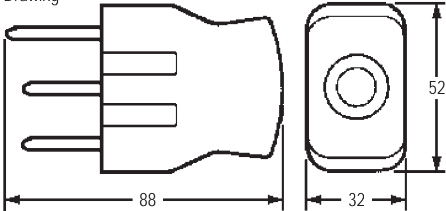
Dimensional Drawing
