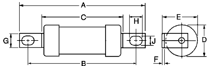
Dimensional Data
